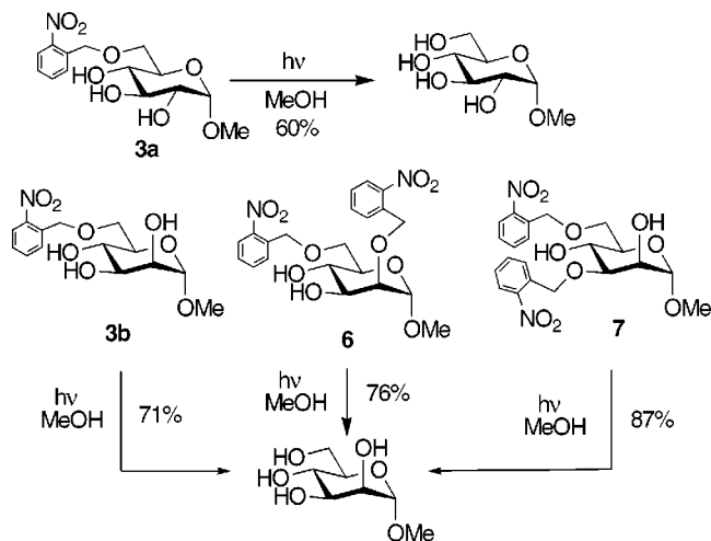
Scheme 3. Deprotection of o -Nitrobenzyl Groups by Irradiation (350 nm) of Photolabile Sugars 3a , 3b , 6 , and 7
